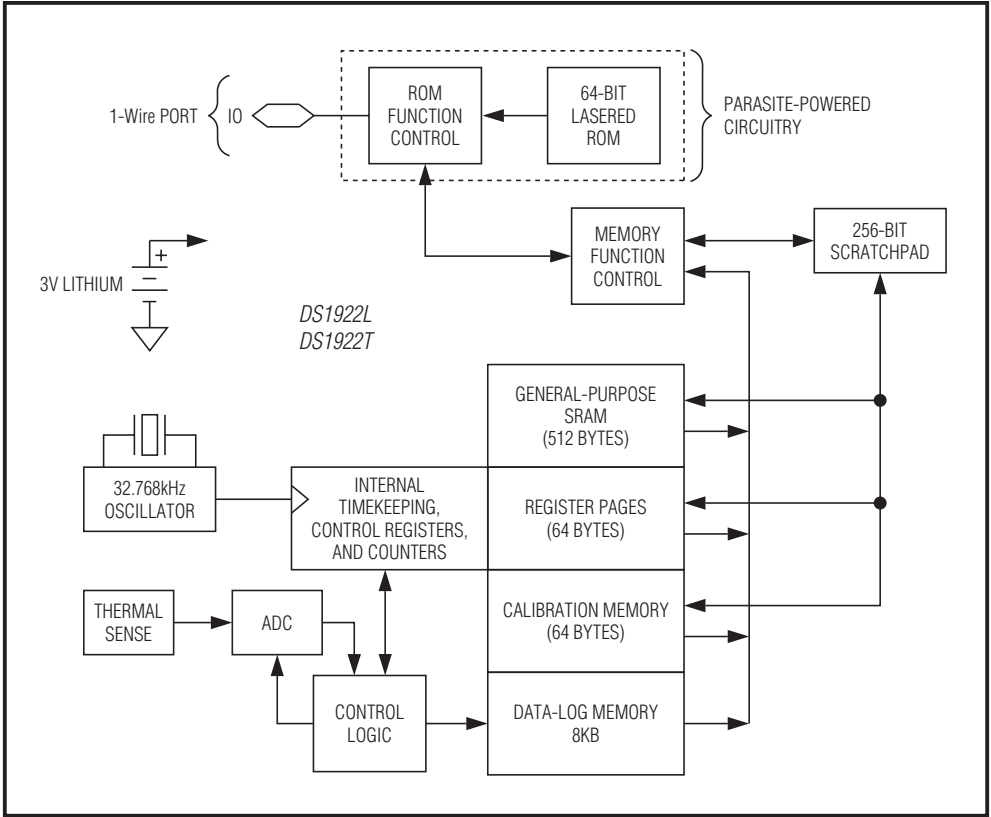
Figure 1. Block Diagram
